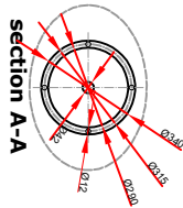
Floor Flange
